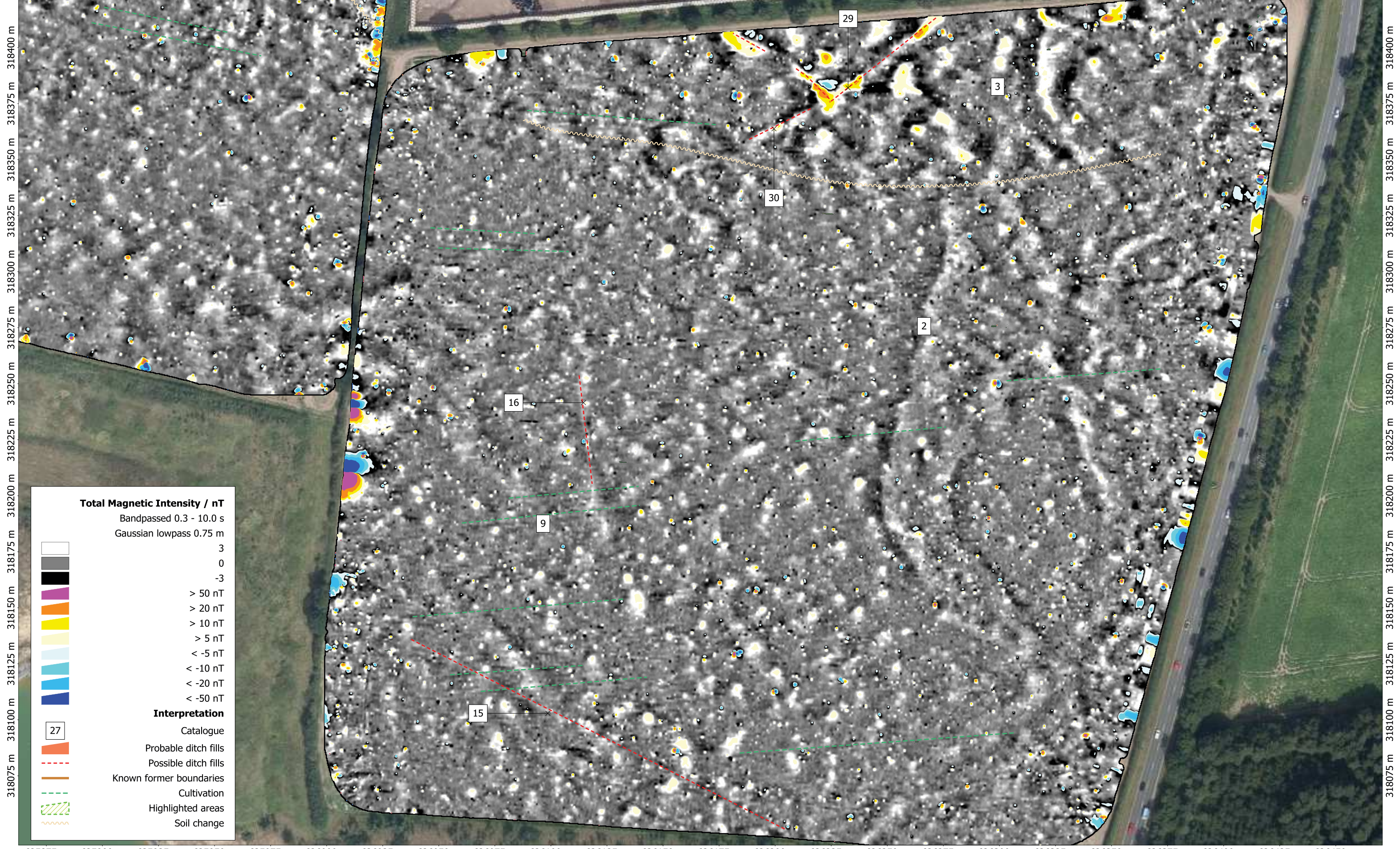
SQH201 Stanninghall Quarry, Horstead, Norfolk DWG 03e Interpretation - Southeast
